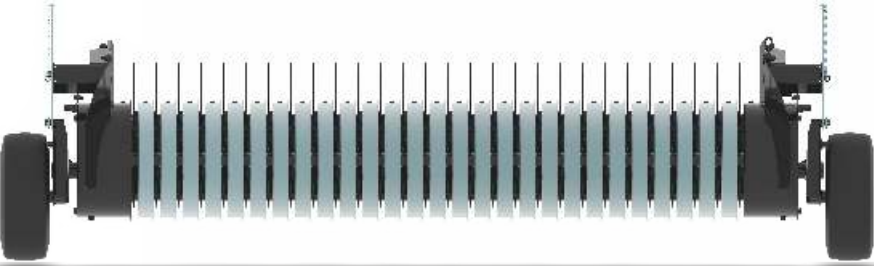
210-cm wide pick-up. Four tine bars. Cut-out clutch and swath roller as standard
