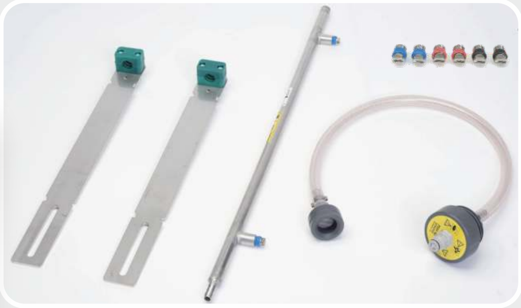
Fan nozzle series. There are three different fan nozzlebars. (with 2 or 3 nozzles for balers, and with 4 nozzles for loading wagons). The delivery tube, fittings, and nozzles are made of stainless steel. The nozzles are colour coded according to the application pattern..
